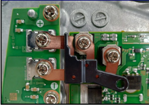
基板間接続 Board to board
