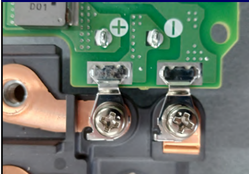
外部接続 Connection with other units
