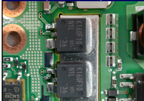
放熱対策(基板表) Heat dissipation measures (Front side)
