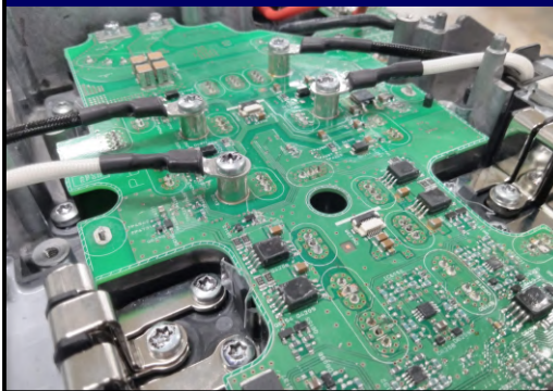
ハーネスとの接続 Connecting SMT spacers and harnesses
