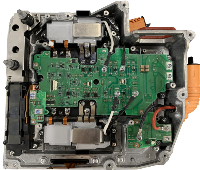
ハーネスとの接続 Connecting SMT spacers and harnesses
