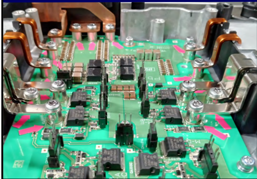
スペーサ実装 Mounting SMT spacers on the metal board
