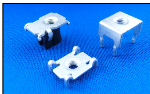
ネジ端子 Screw terminal
